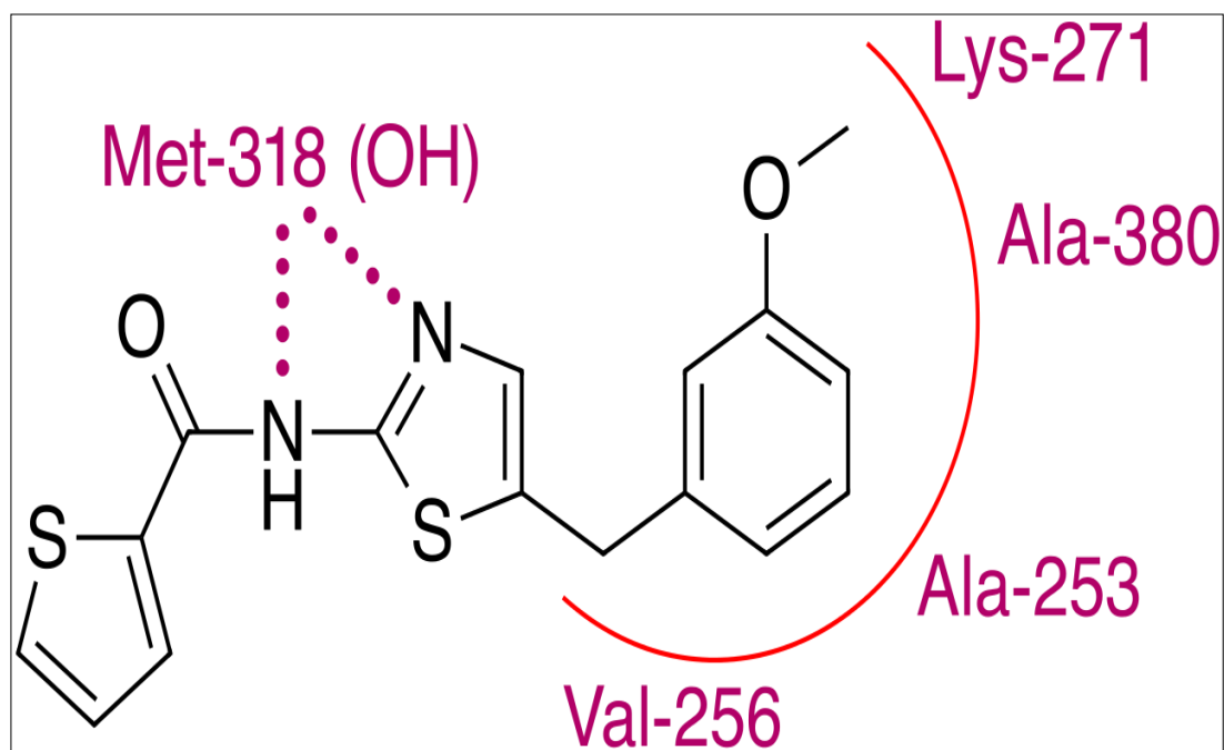
Figure 9. Proposed binding site interactions of substance.
